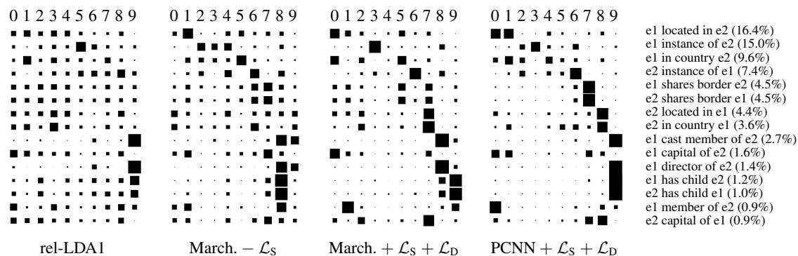
Figure 3: Normalized contingency tables for the TReX SPO dataset. Each of the 10 columns corresponds to a predicted relation cluster, which were sorted to ease comparison. The rows identify Wikidata relations sorted by frequency in the TReX SPO corpus. The area of each square is proportional to the number of sentences in the cell. The matrix was normalized so that each row sum to 1, thus it is more akin to a B^3 per-item recall than a true contingency table.
